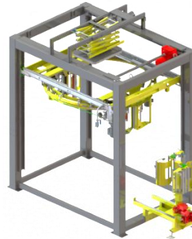
Octopus 1850T
